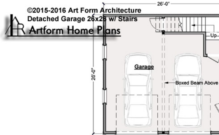
Area this Floor: 676 sq ft 9'-9" Ceiling Ht.
